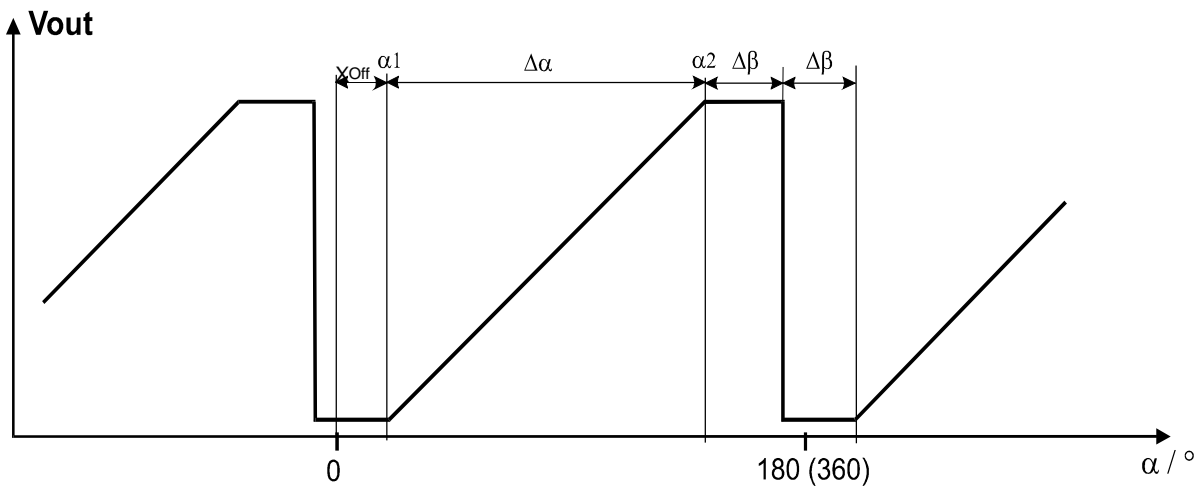
Figure 14: Output curve for different angular ranges including a zero point offset. Note that when using MR-sensors (KMZ41), the signal period is 0° to 180° as the signals are proportional to \sin 2\alpha and \cos 2\alpha .
