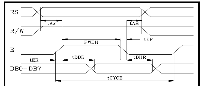
Read Operation
