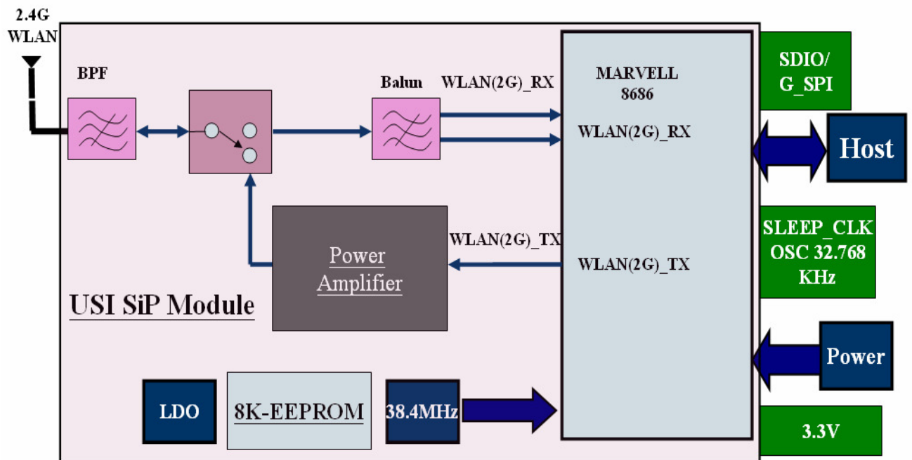
Fig. WM-G-MR-10 Block Diagram
