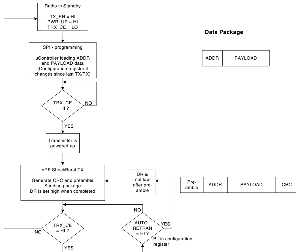
Figure 3 Flowchart ShockBurst™ transmit of nRF905.
