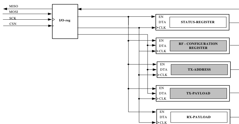
Figure 5 SPI – interface and the five internal registers.
