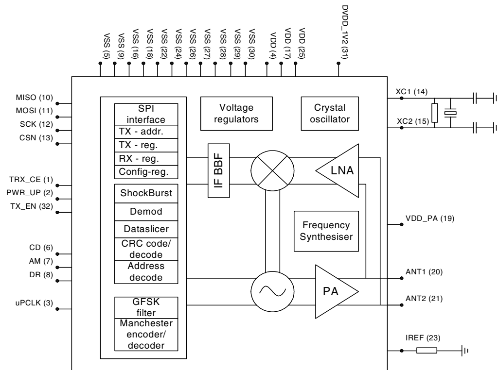
Figure 1 nRF905 with external components.
