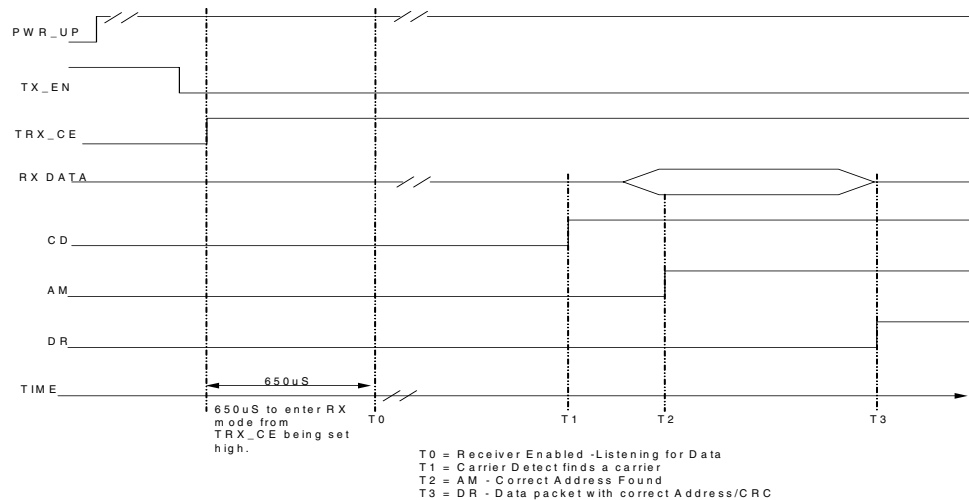
Figure 10 Timing diagram for standby to receiving.
