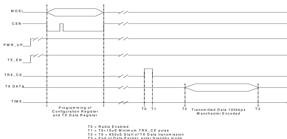
Figure 9 Timing diagram for standby to transmit.
