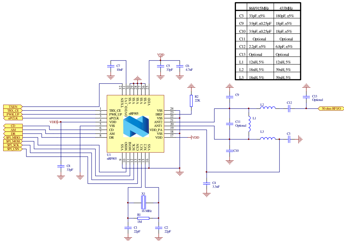
Figure 15 nRF905 Application schematic, single ended connection to 50Ω antenna by using a differential to single ended matching network.
