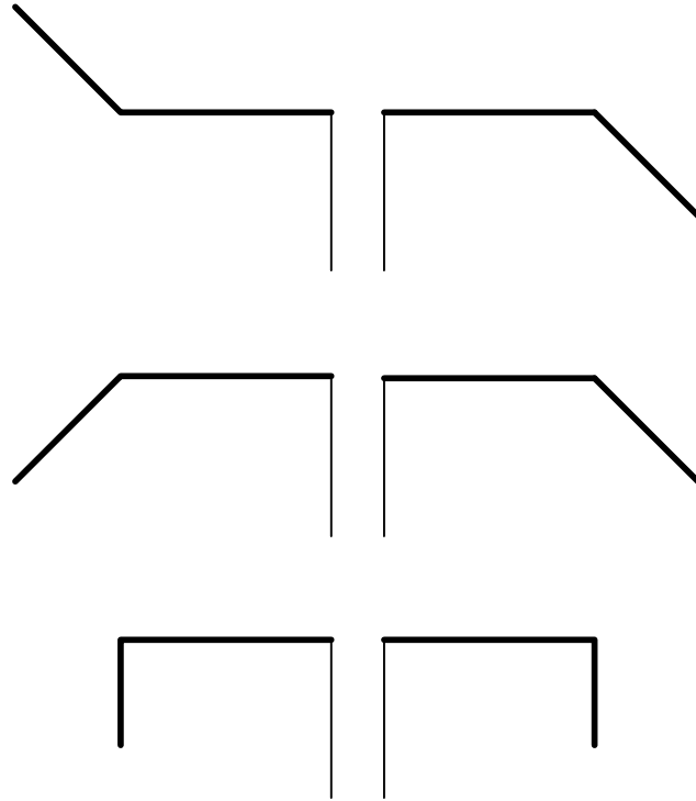
Figure 2. Dipole Shapes to Improve Omnidirectional Characteristics
