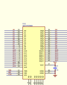
RAM & FLASH
