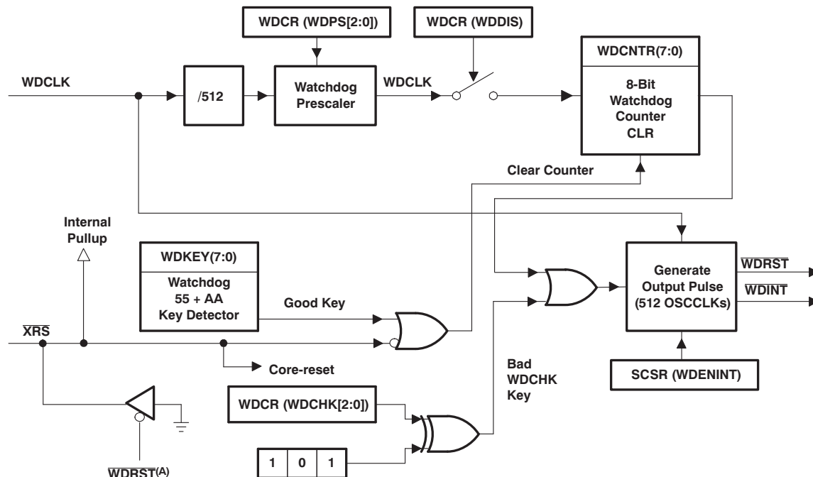
Figure 3-14. CPU-watchdog Module
