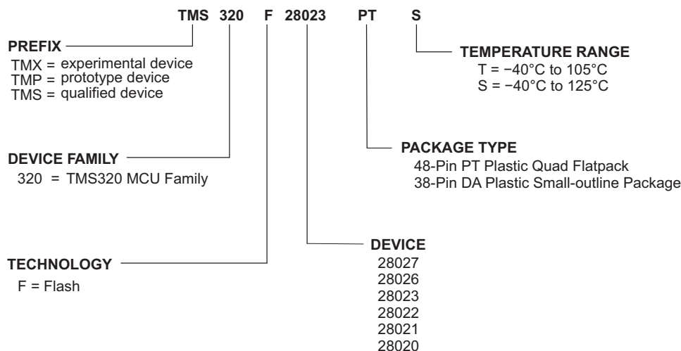
Figure 5-1. Device Nomenclature
