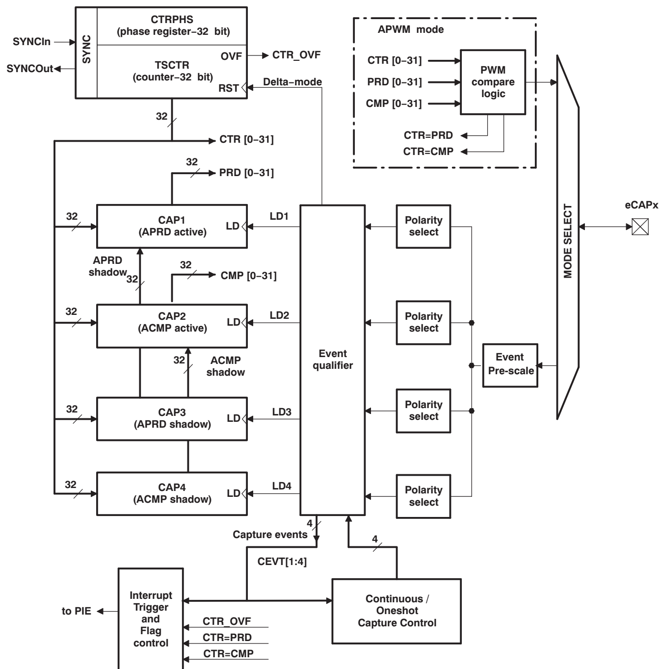
The eCAP module is clocked at the SYSCLKOUT rate.
