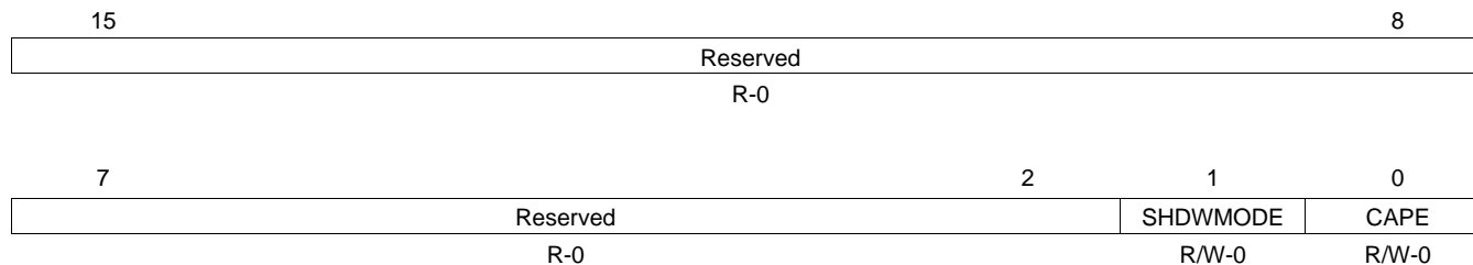
Figure 4-36. Digital Compare Capture Control Register (DCCAPCTL)
