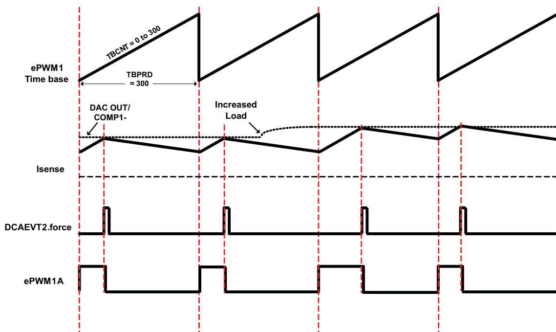
Figure 3-18. Peak Current Mode Control Waveforms for Figure 3-17
