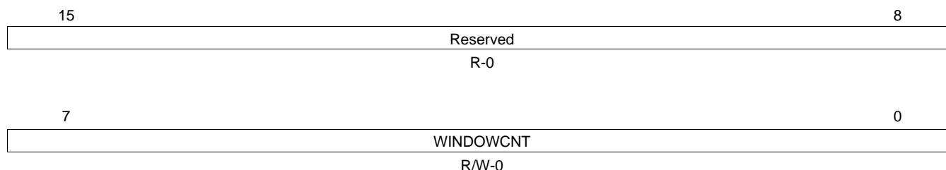
Figure 4-41. Digital Compare Filter Window Counter Register (DCFWINDOWCNT)
