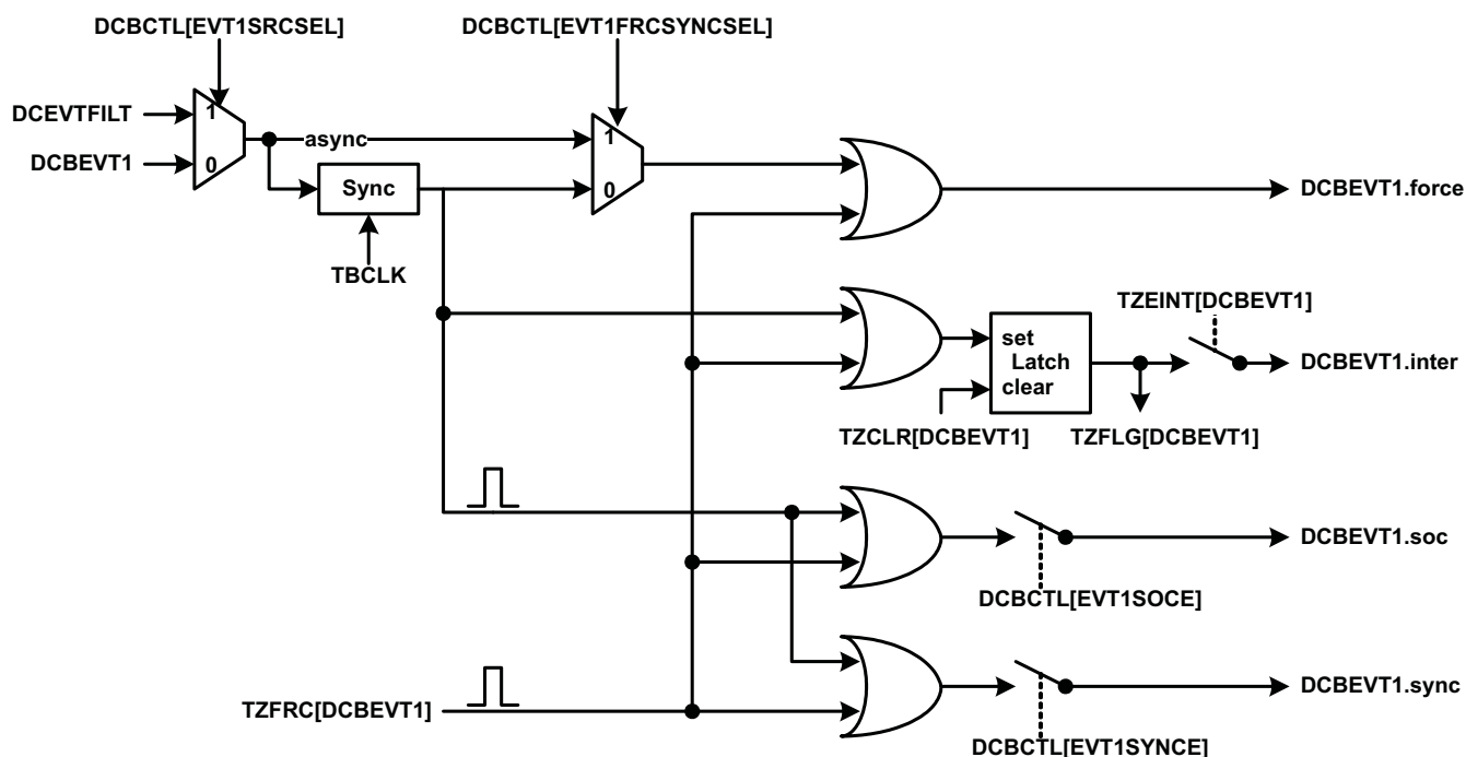
Figure 2-47. DCBEVT1 Event Triggering
