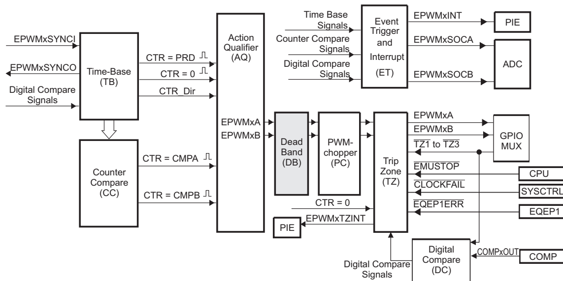
Figure 2-27. Dead_Band Submodule
