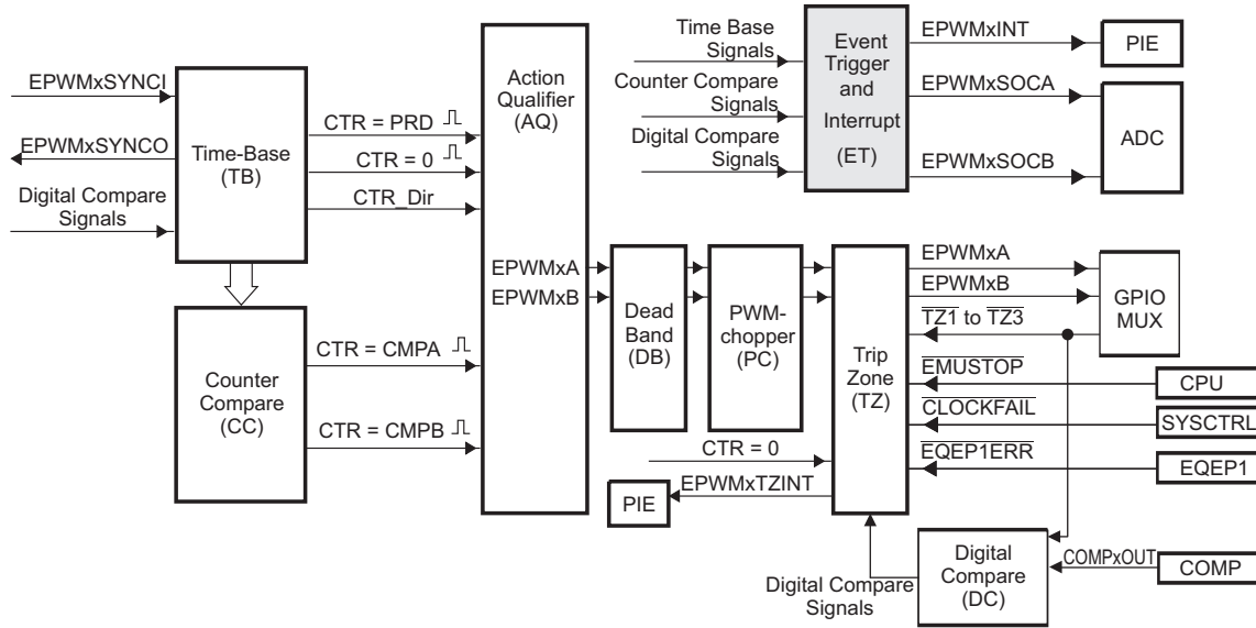
Figure 2-38. Event-Trigger Submodule
