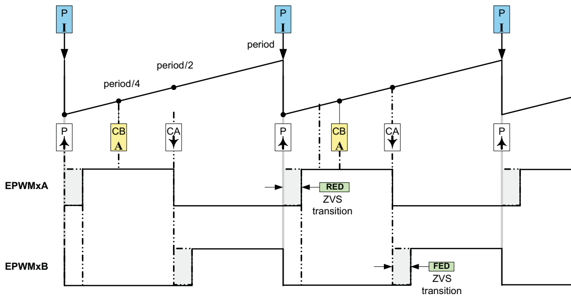
Figure 3-20. H-Bridge LLC Resonant Converter PWM Waveforms
