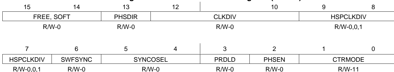
Figure 4-8. Time-Base Control Register (TBCTL)
