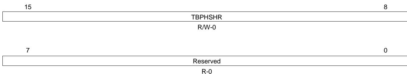
Figure 4-6. Time-Base Phase High Resolution Register (TBPHSHR)
