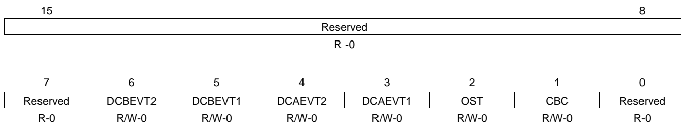
Figure 4-27. Trip-Zone Enable Interrupt Register (TZEINT)
