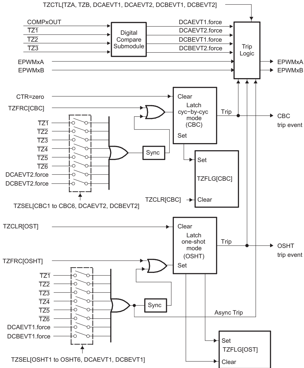
Figure 2-36. Trip-Zone Submodule Mode Control Logic
