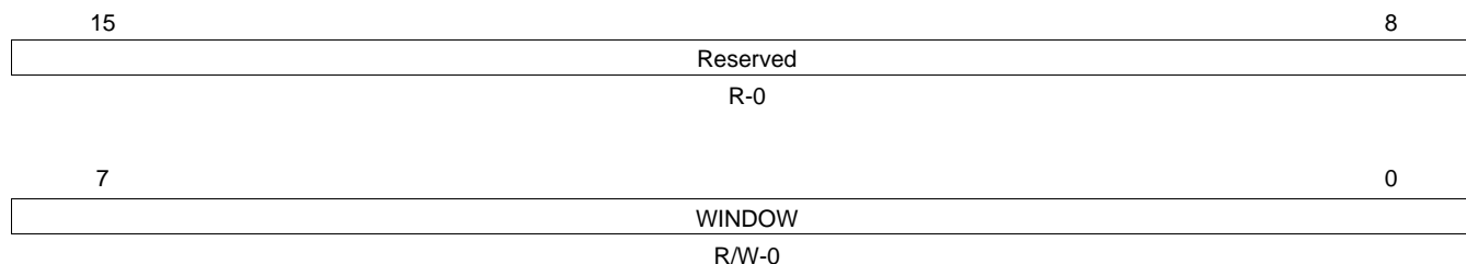
Figure 4-40. Digital Compare Filter Window Register (DCFWINDOW)
