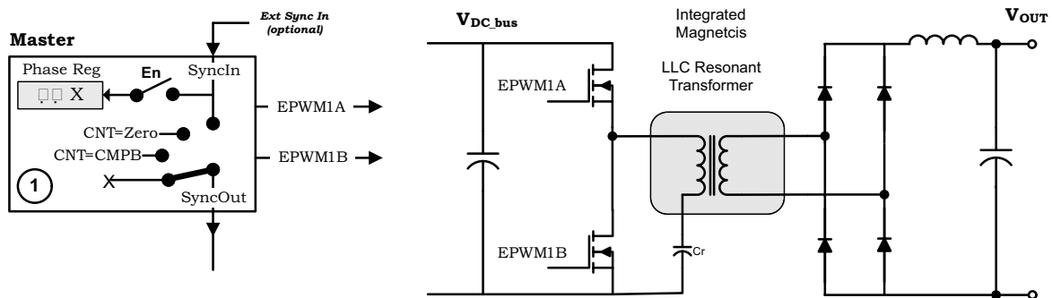
Figure 3-19. Control of Two Resonant Converter Stages
