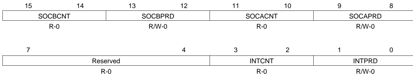
Figure 4-43. Event-Trigger Prescale Register (ETPS)
