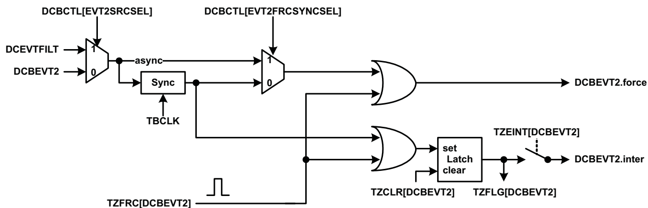
Figure 2-48. DCBEVT2 Event Triggering
