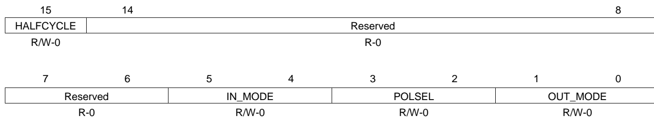
Figure 4-21. Dead-Band Generator Control Register (DBCTL)
