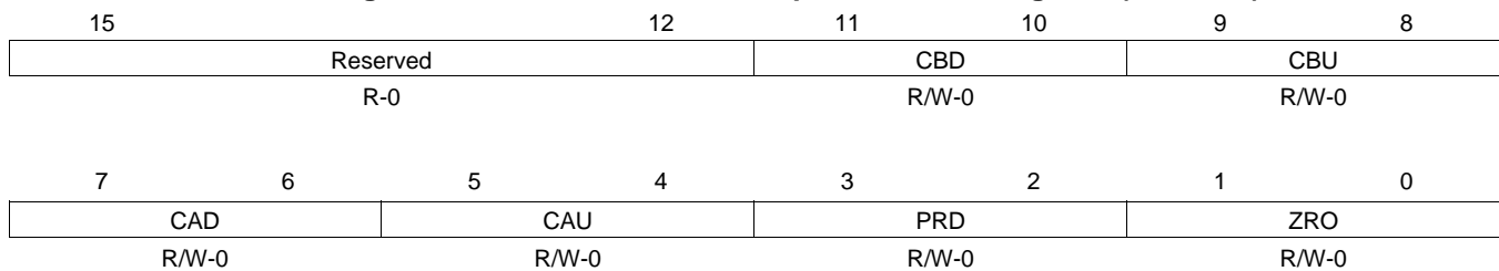
Figure 4-18. Action-Qualifier Output B Control Register (AQCTLB)
