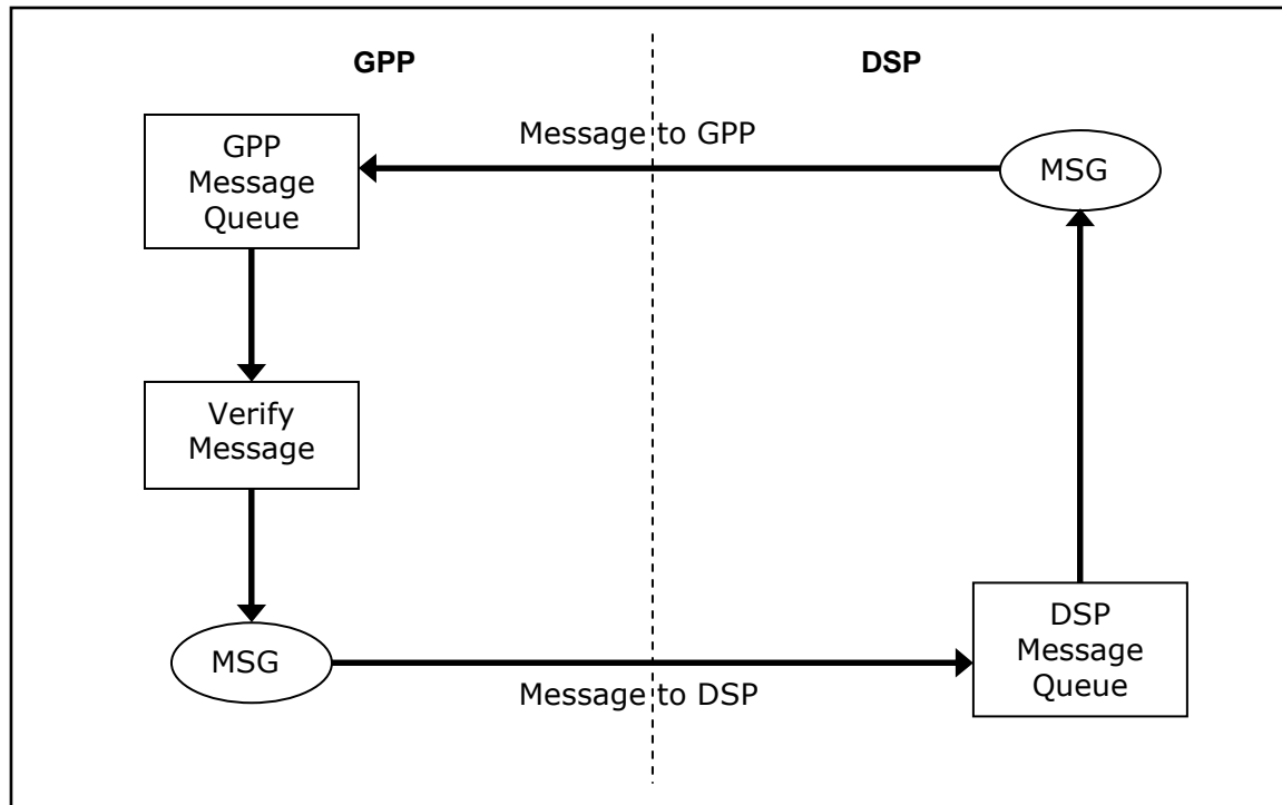
Figure7. Messageflowinthesampleapplication–MESSAGE
