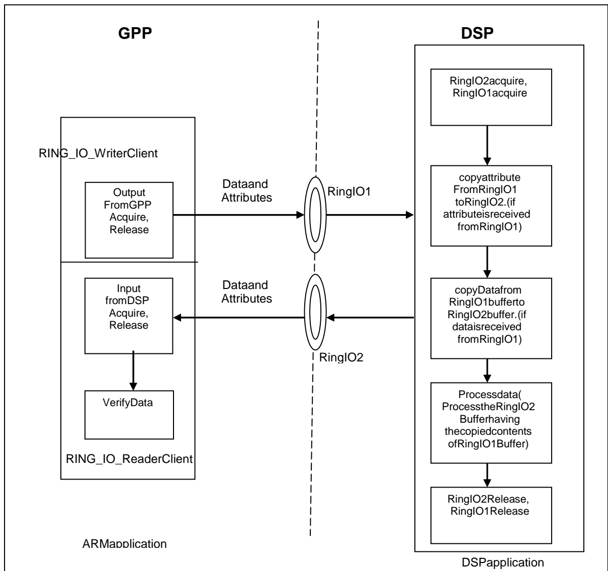
Figure 11. Data flow in the sample application—RING_IO
