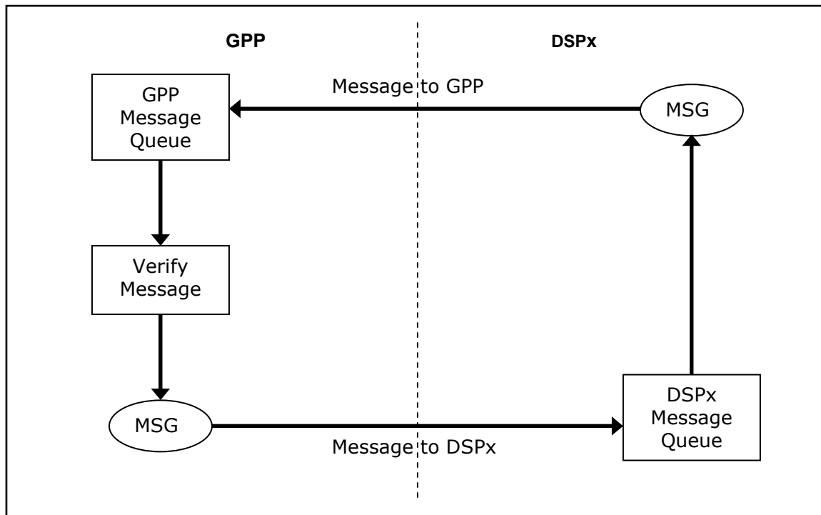
Figure15. Messageflowinthesampleapplication–MESSAGE
