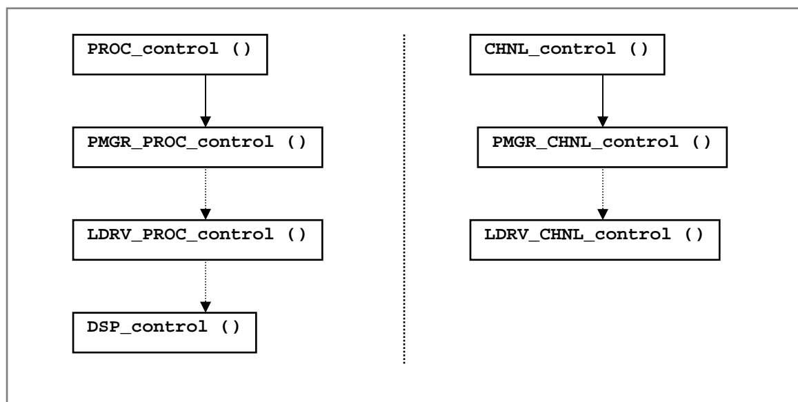
Figure17. Executionflow:PROC_control()andCHNL_control()
