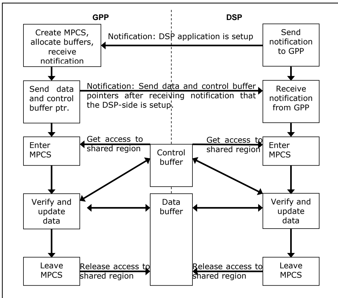
Figure13. Dataflowinthesampleapplication–MPCSXFER
