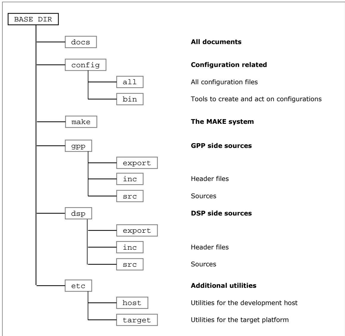
Figure2. Toplevelviewofdirectorystructure
