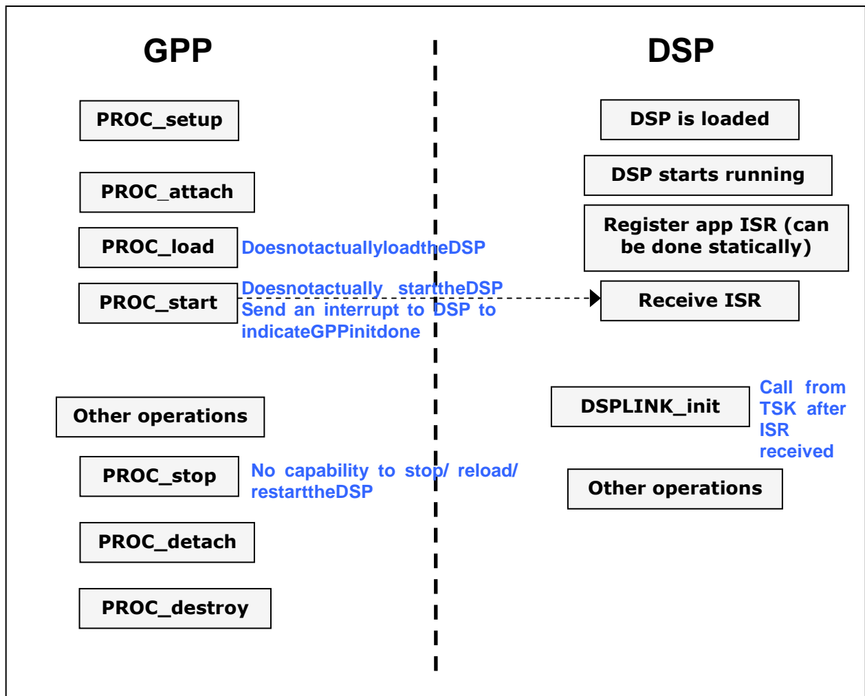
Figure 6. ExternalLoadAndStartMode
