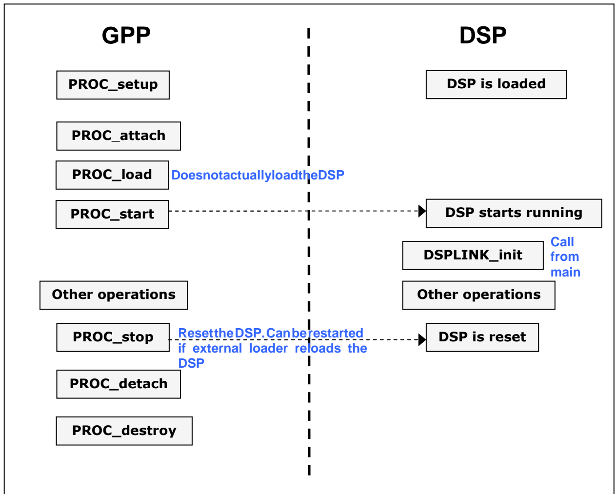
Figure5. ExternalLoadMode
