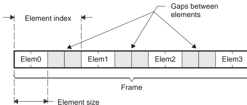
Figure 1-5. Transfer Properties for 1-D Frame
