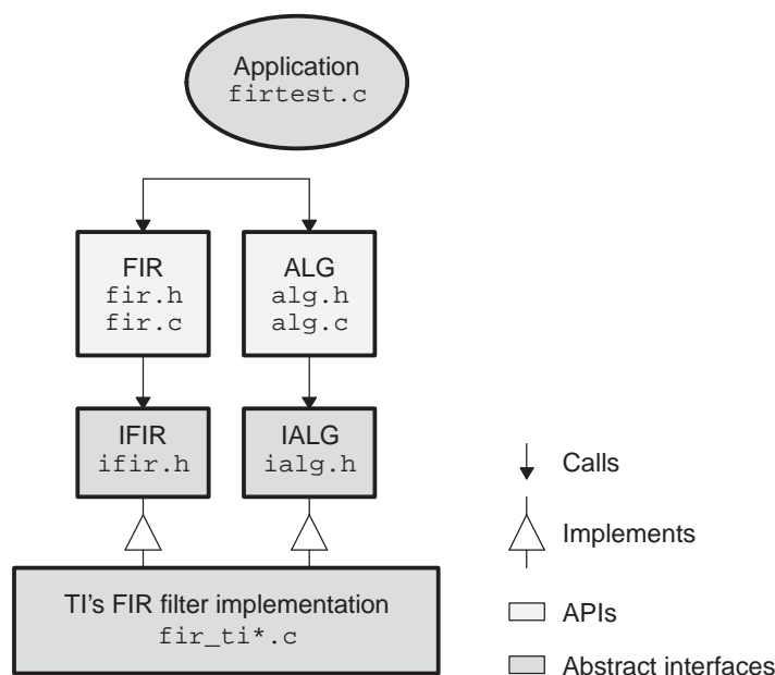
Figure A-1. FIR Filter Example Implementation
