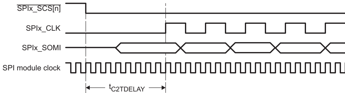
Figure 29. Example: t_{\text{C2TDELAY}} = 8 SPI Module Clock Cycles
