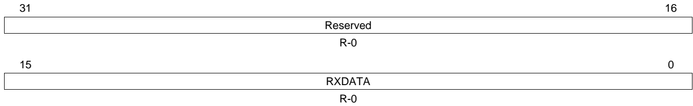
Figure 27. SPI Emulation Register (SPIEMU)
