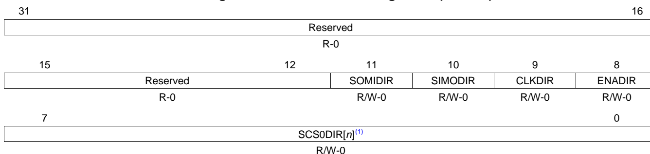
Figure 19. SPI Pin Control Register 1 (SPIPC1)
