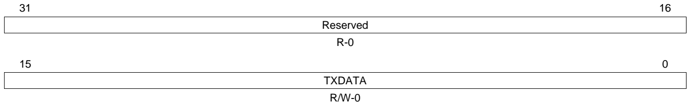
Figure 24. SPI Data Register 0 (SPIDAT0)
