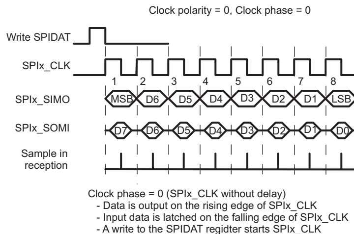
Figure 8. Clock Mode with POLARITY = 0 and PHASE = 0
