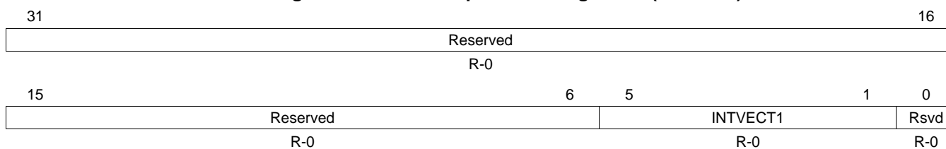
Figure 35. SPI Interrupt Vector Register 1 (INTVEC1)
