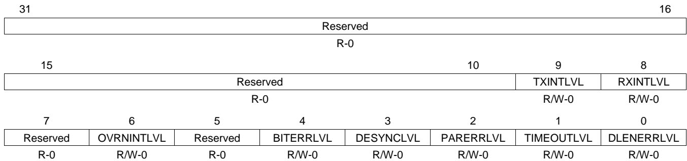
Figure 16. SPI Interrupt Level Register (SPILVL)
