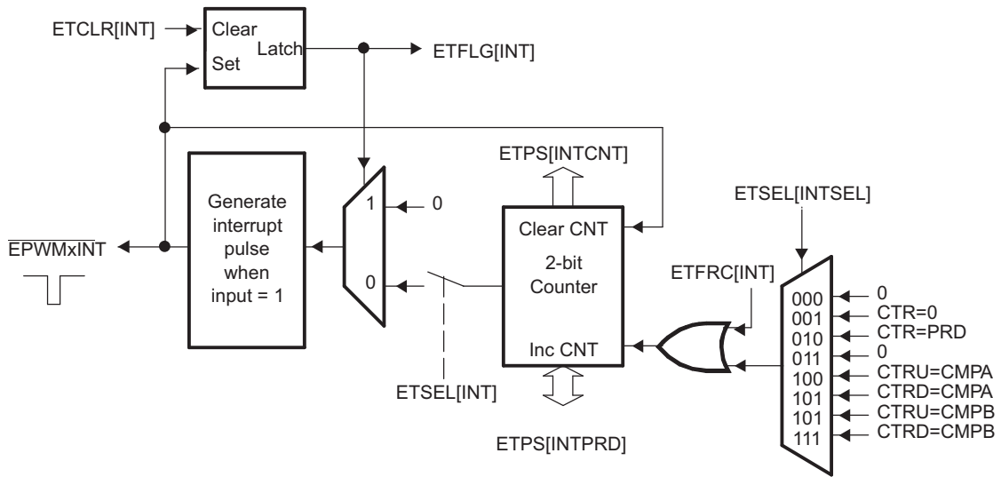
Figure 42. Event-Trigger Interrupt Generator
