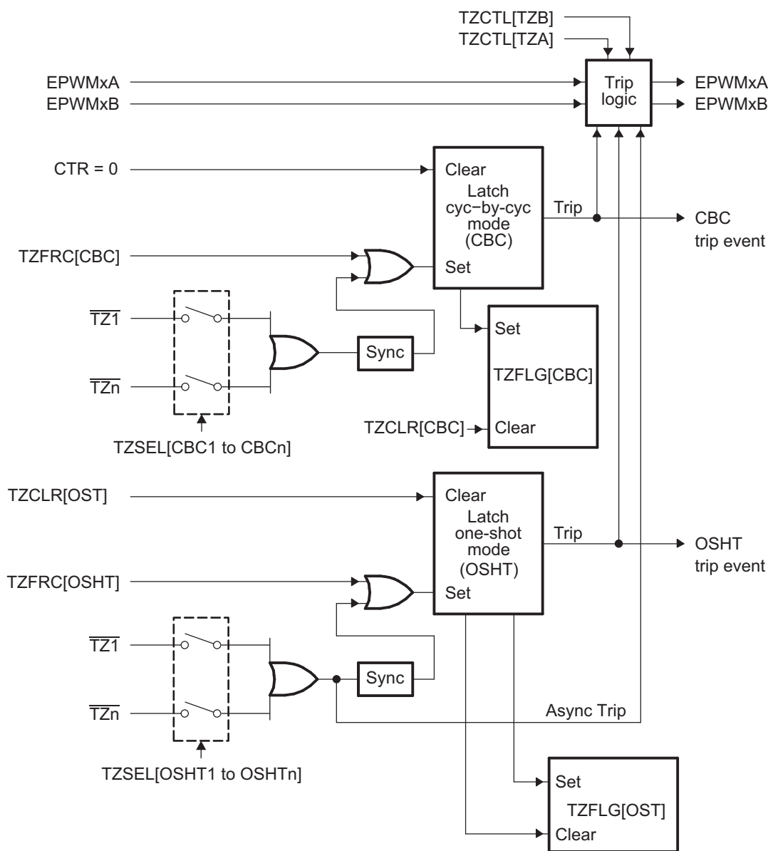
Figure 37. Trip-Zone Submodule Mode Control Logic
