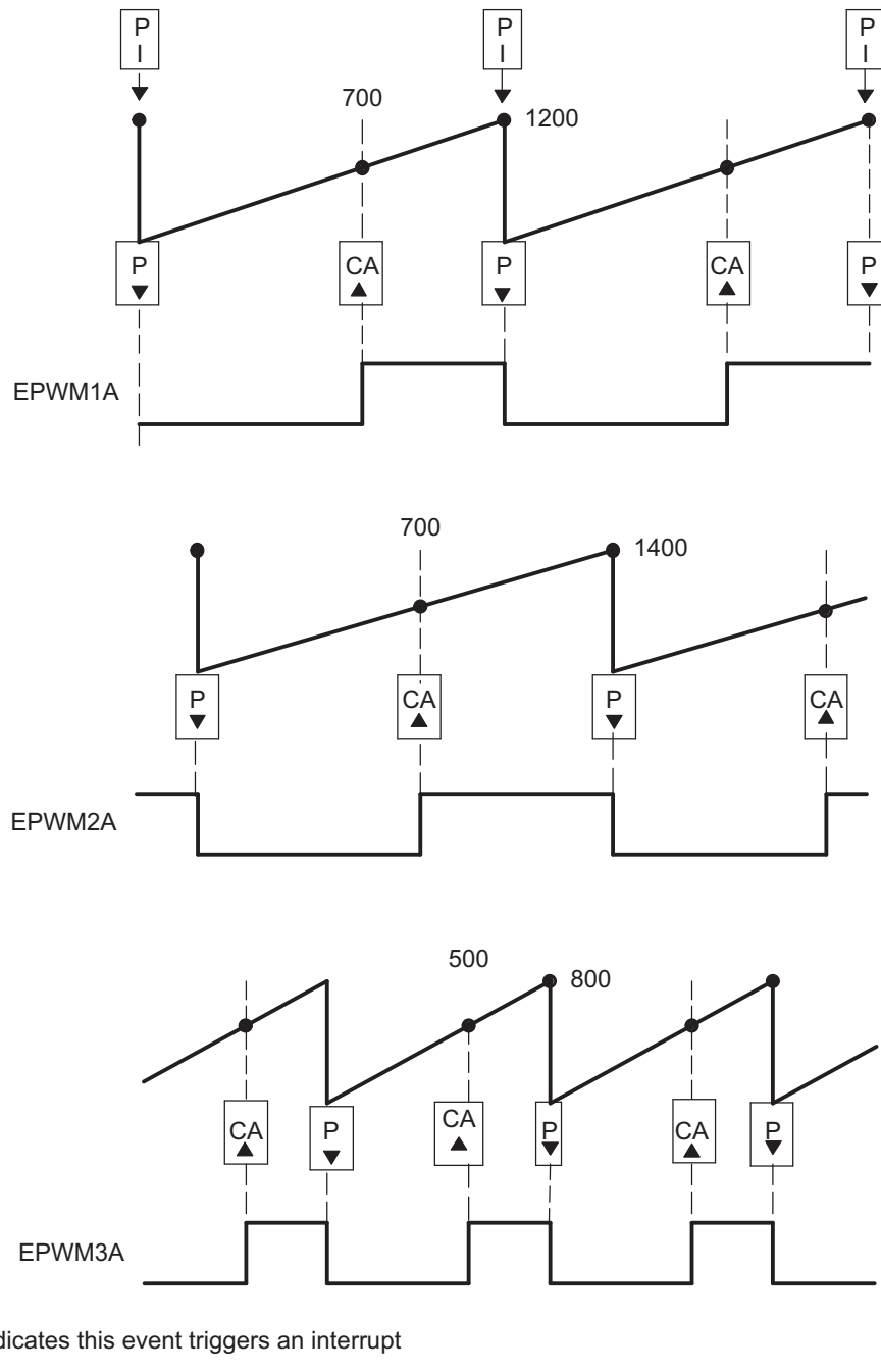
Figure 52. Buck Waveforms for Figure 51 (Note: Only three bucks shown here)
