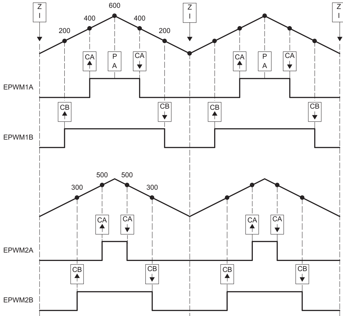
Figure 54. Buck Waveforms for Figure 53 (Note: F_{PWM2} = F_{PWM1} )
