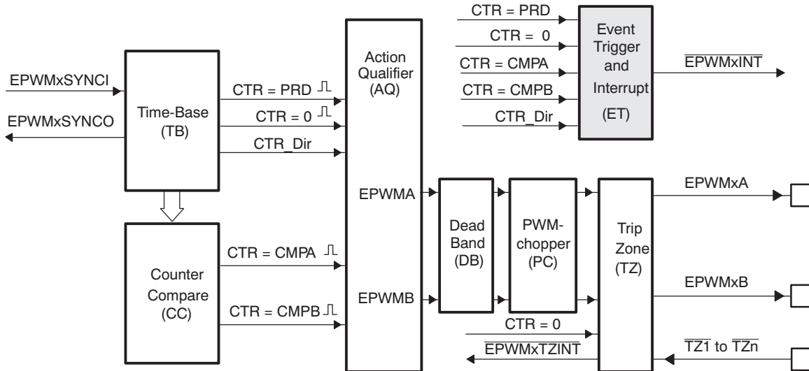
Figure 39. Event-Trigger Submodule
