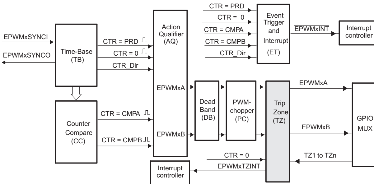
Figure 36. Trip-Zone Submodule
