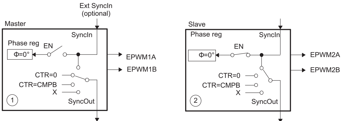
Figure 50. EPWM1 Configured as a Typical Master, EPWM2 Configured as a Slave
