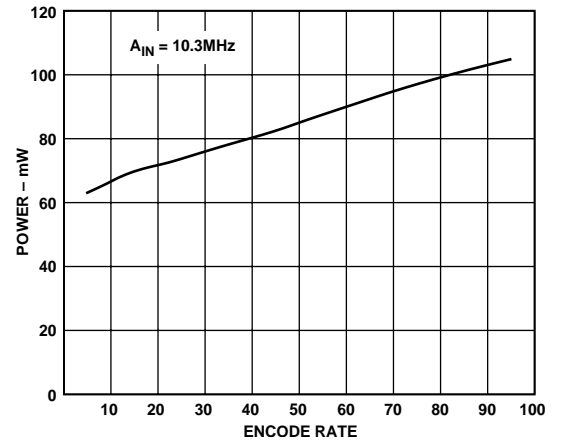
Figure 16. Analog Power Dissipation vs. Encode Rate
