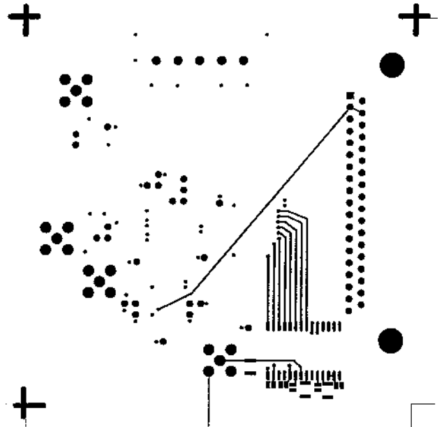
Figure 25. Printed Circuit Board Bottom Side Copper
