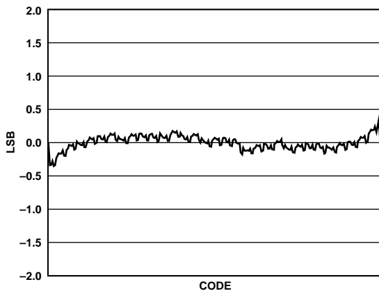
Figure 19. Integral Nonlinearity
