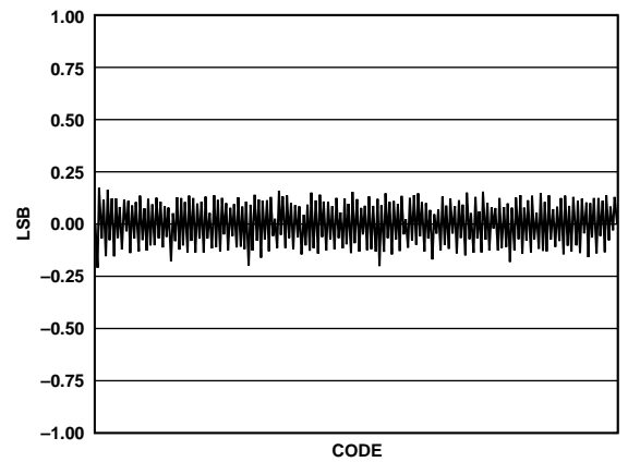
Figure 18. Differential Nonlinearity
