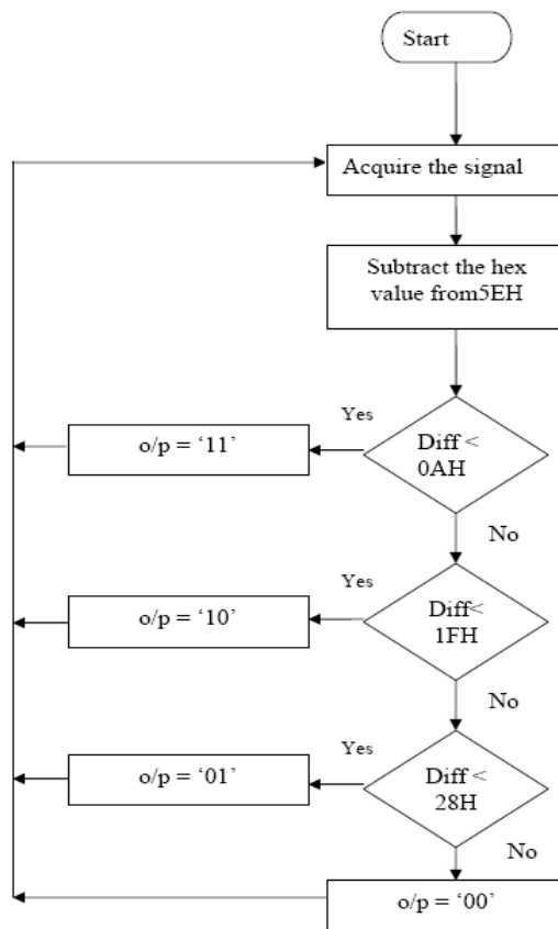
Fig. 2 Adaptive power control Algorithm Flow chart
