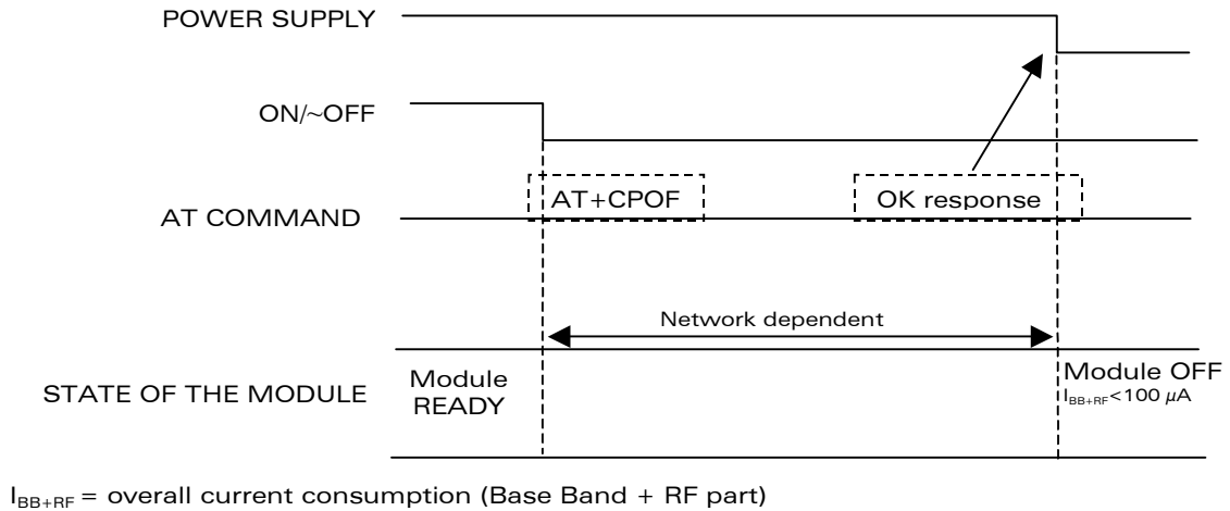
Figure 5: Power-OFF sequence diagram
