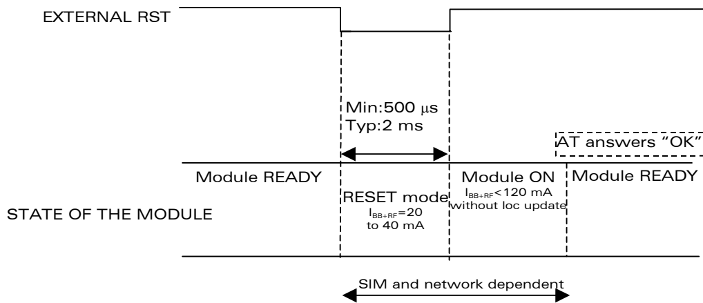
Figure 6: Reset sequence diagram
