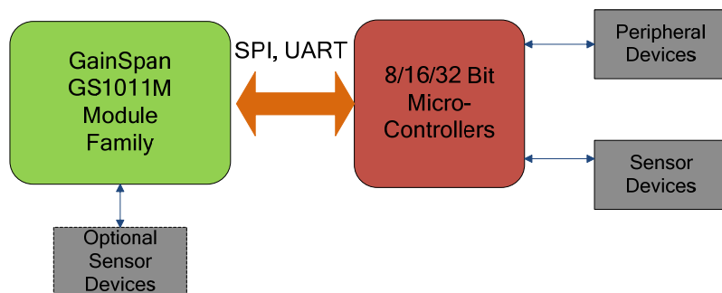
GS1011M based Embedded Design
