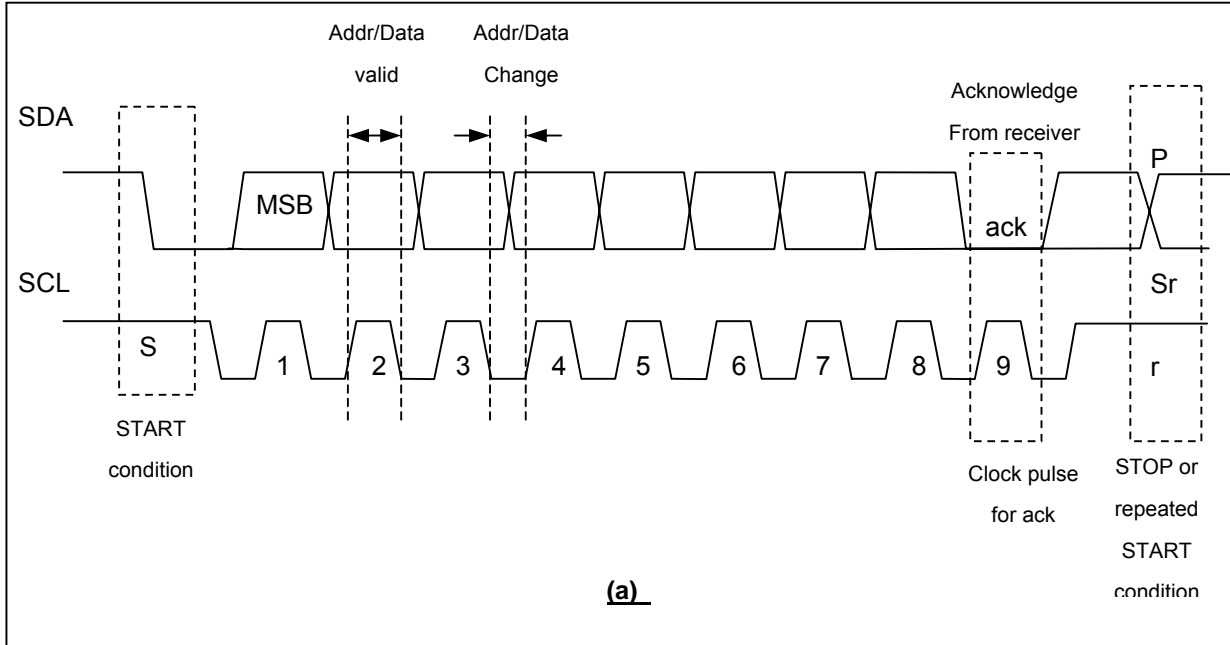
Figure 17-1 I2C-bus Protocol
