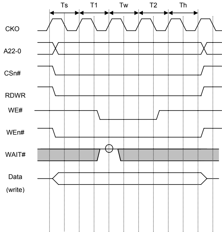
Figure 3-12 Byte Control SRAM Write Timing
