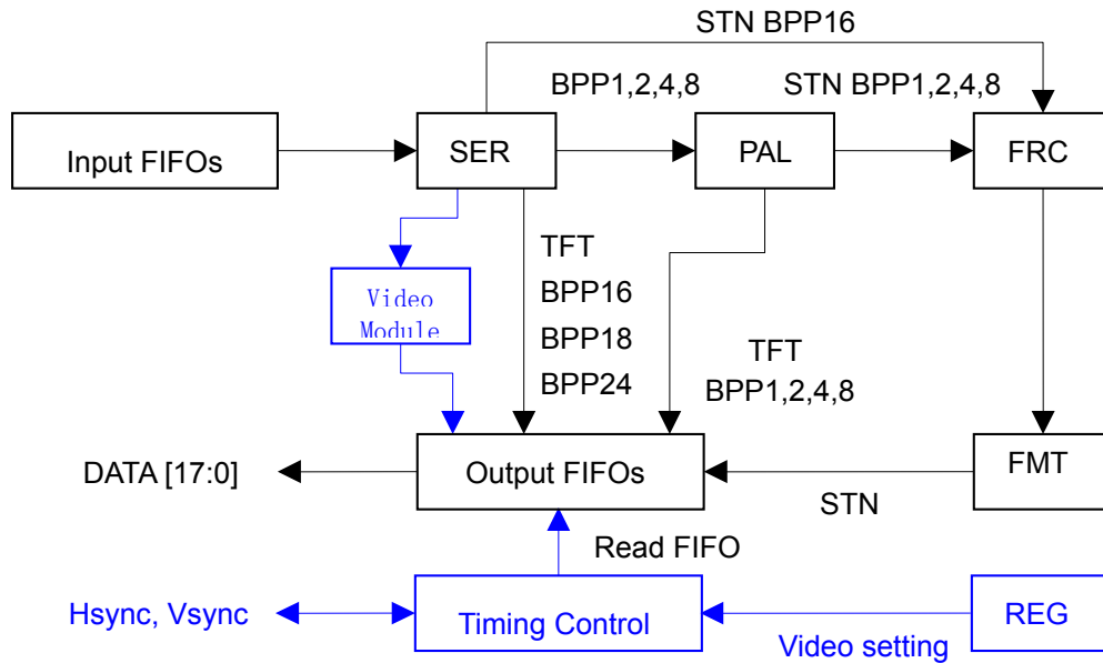
Figure 11-1 Block Diagram
