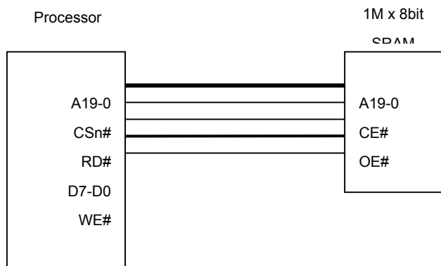
Figure 3-4 Example of 8-Bit Data Width SRAM Connection
