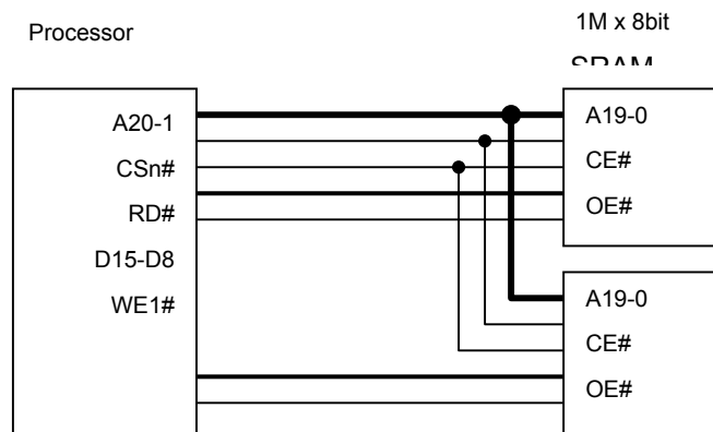
Figure 3-3 Example of 16-Bit Data Width SRAM Connection
