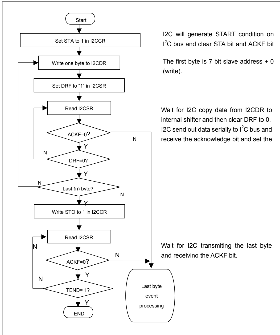
Figure 17-9 I2C Write Operation Flowchart
