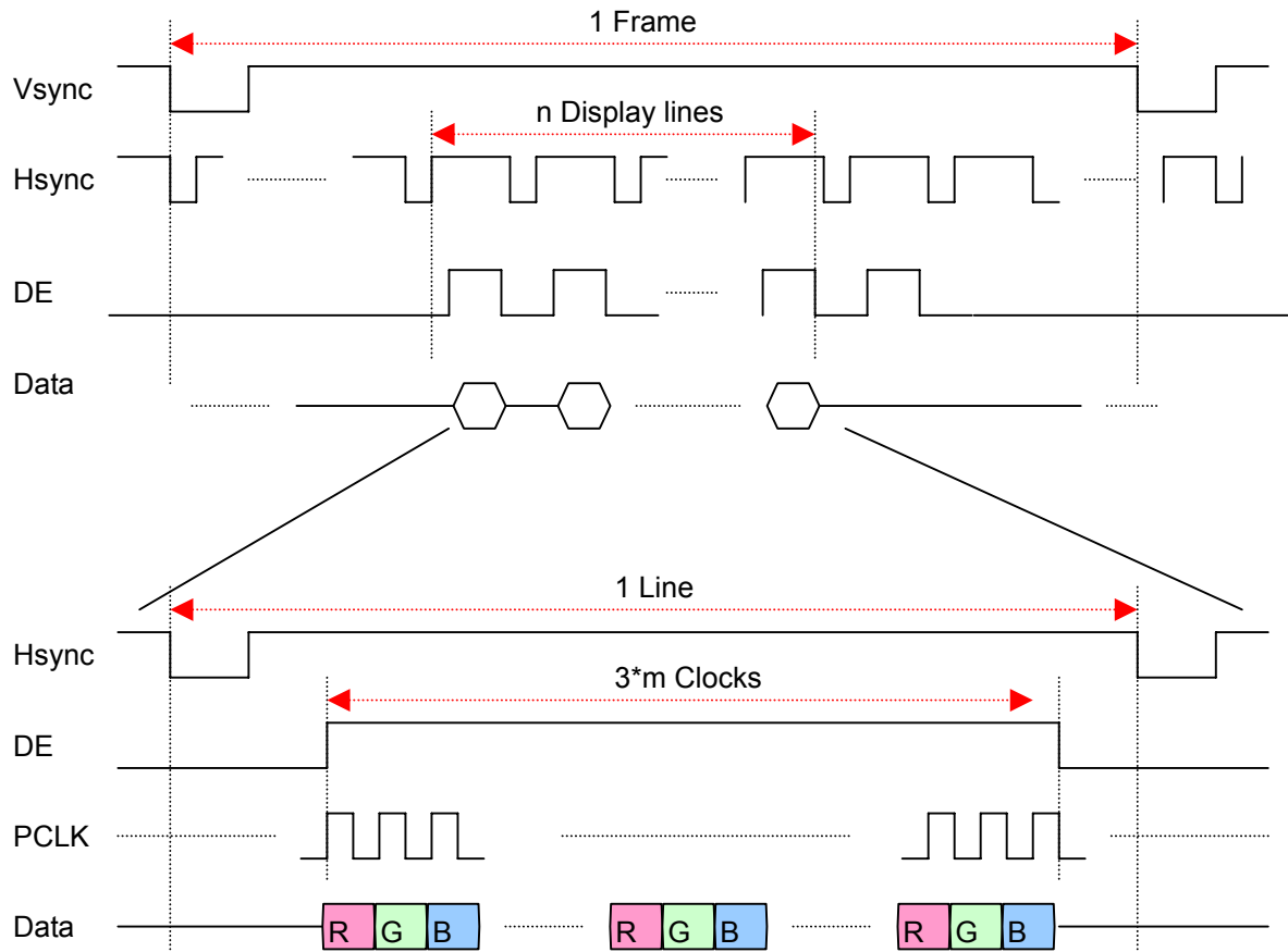
Figure 11-3 8-bit serial TFT LCD Timing (24bpp)
