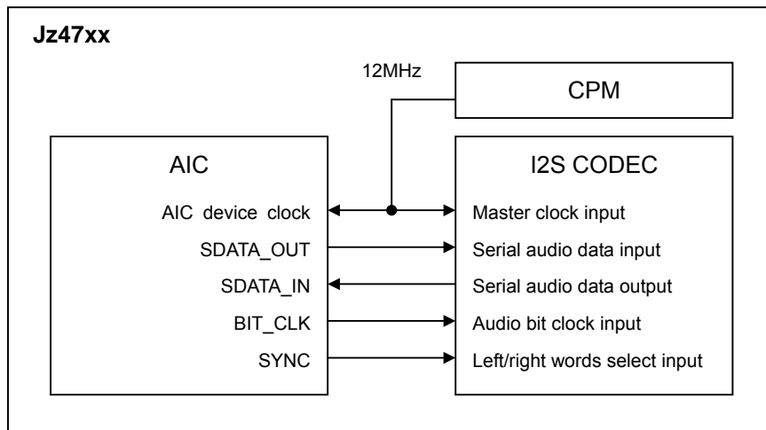
Figure 13-2 Interface to the Internal I2S CODEC Diagram
