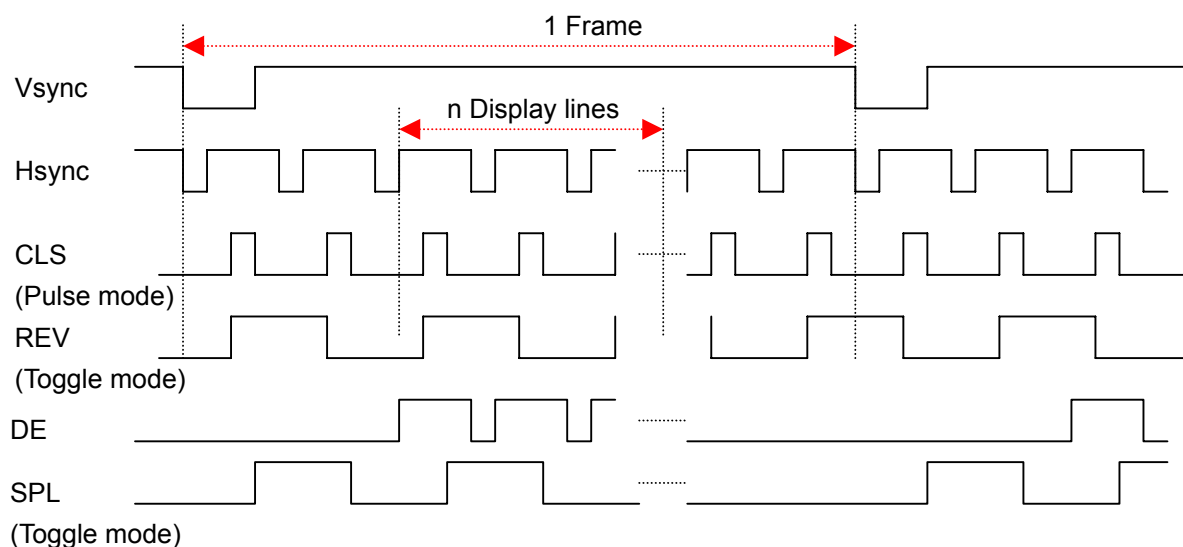
Figure 11-3 Special TFT LCD Timing 1
