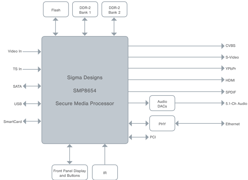
Block Diagram of Vantage 8654
