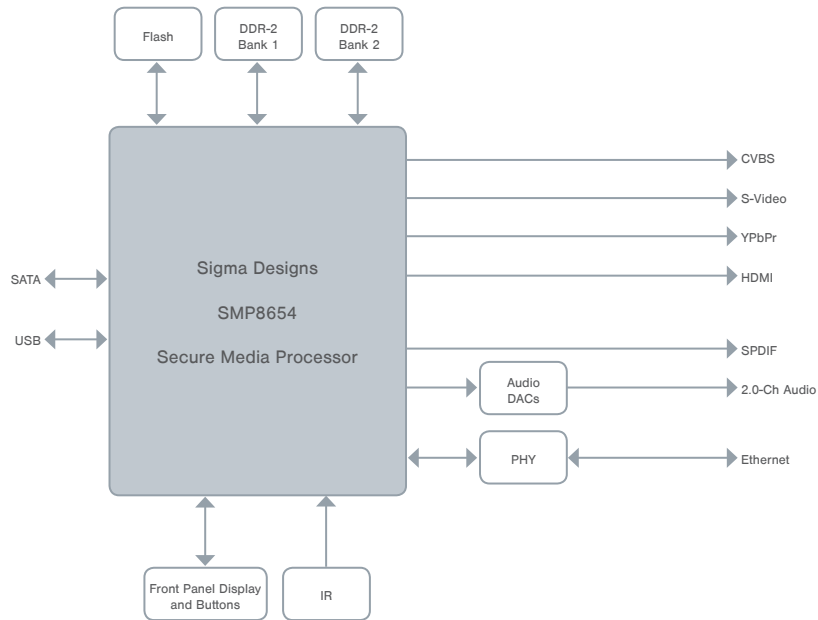
Block Diagram of IPTV-8654
