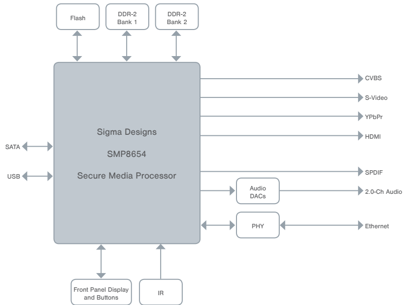
Block Diagram of DMA-8654
