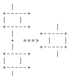
Figure 28a – A sequence consisting of a step, a transition and a step is replaced by one step
