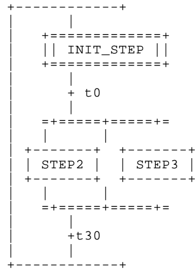
Figure 29b – No reduction required per termination rule 2
