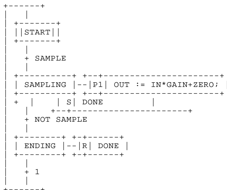
Figure 19 – Example of incorrect and allowed programming constructs
