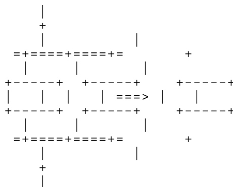
Figure 28d – A simultaneous sequence (AND branch) is replaced by one step
