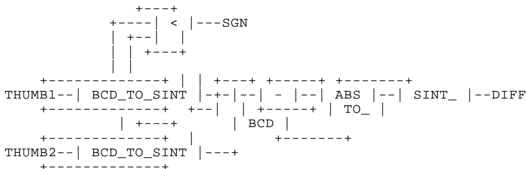
Figure 4b – Body Figure 4 – Function block BCD DIFF
