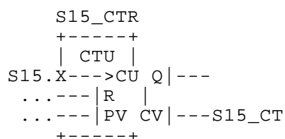
Figure 17d – Correct body for action A15 (FBD language)
