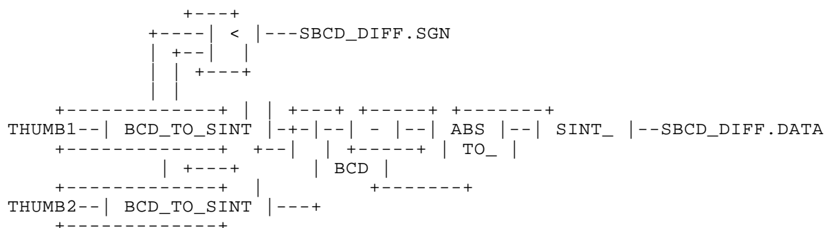
Figure 5c – Body Figure 5 – Function block SBCD_DIFFF
