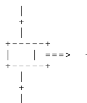
Figure 28b – A sequence consisting of a transition, a step and a transition is replaced by one transition
