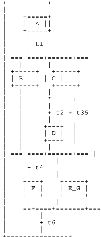
Figure 29d – An irreducible (unreachable) SFC
