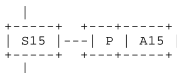
Figure 17a – SFC fragment
