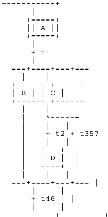
Figure 29c – An irreducible (unsafe) SFC
