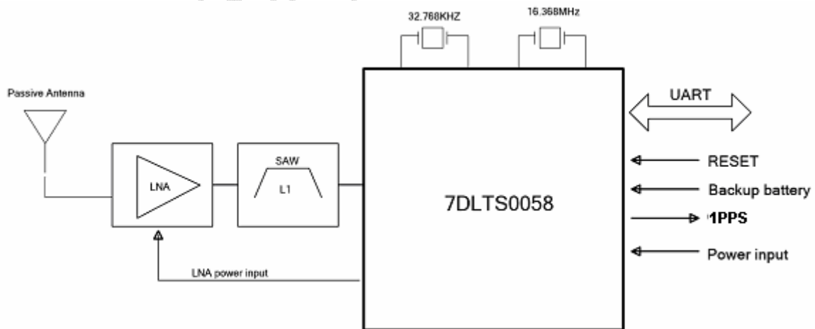
Figure 1 Module architecture
