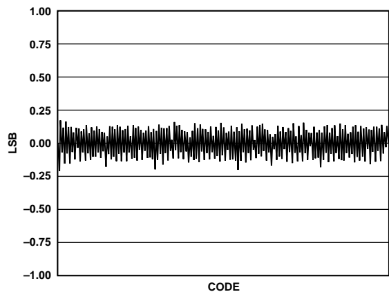
Figure 17. Differential Nonlinearity
