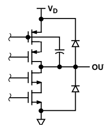
Figure 23. Equivalent Reference Output Circuit
