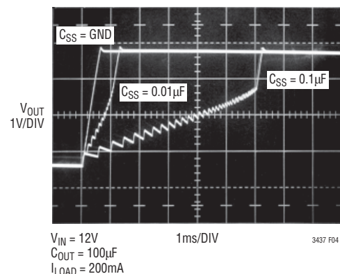
Figure 4. V_{OUT} dV/dt
