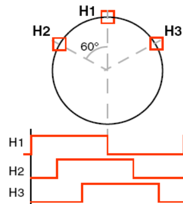
3 Sensor 60^\circ
