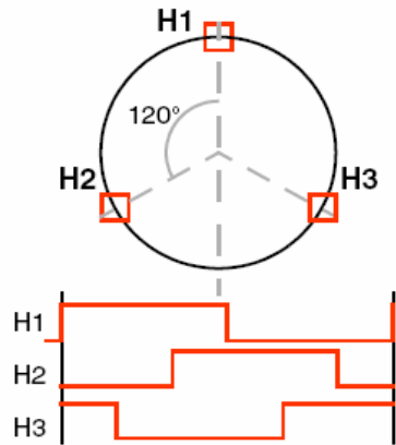
3 Sensor 120^\circ
